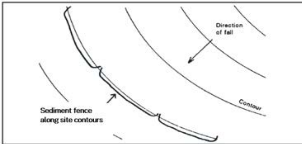
Figure 10. Sediment fence placed along site contours. Source: Adapted from Managing Urban Stormwater: Soils and Construction , 4th edition
