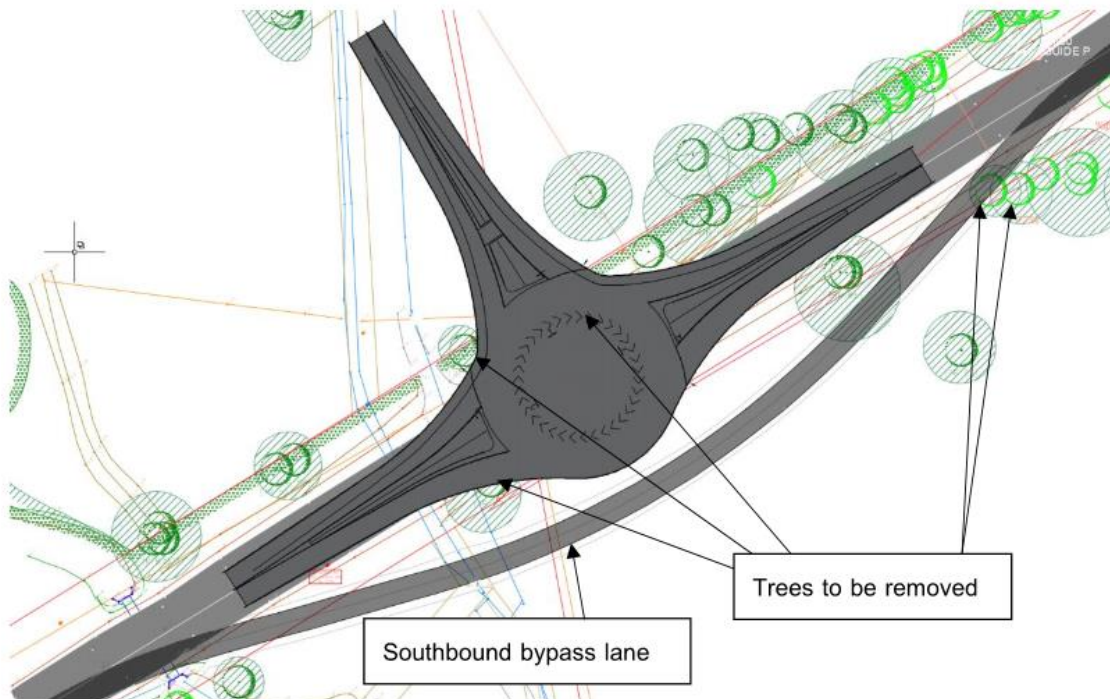
Figure 25: Option B Concept Layout (from Ingen Consulting).
